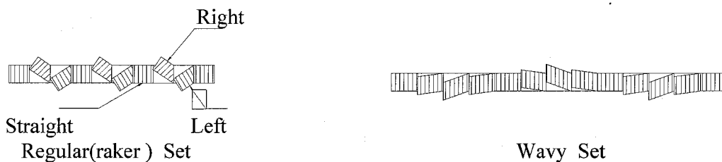
Fig. 7.1 The saw set
